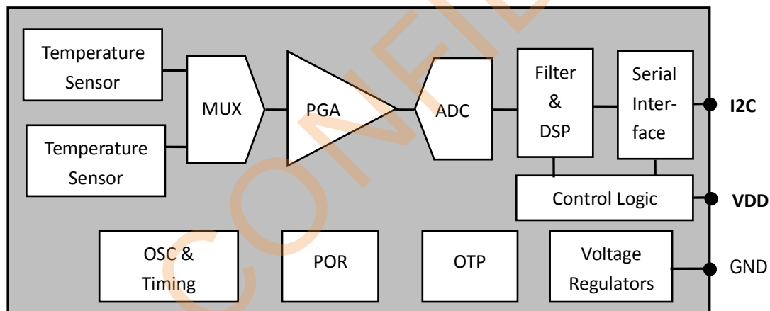
Figure 1 Block diagram of WF5837F
