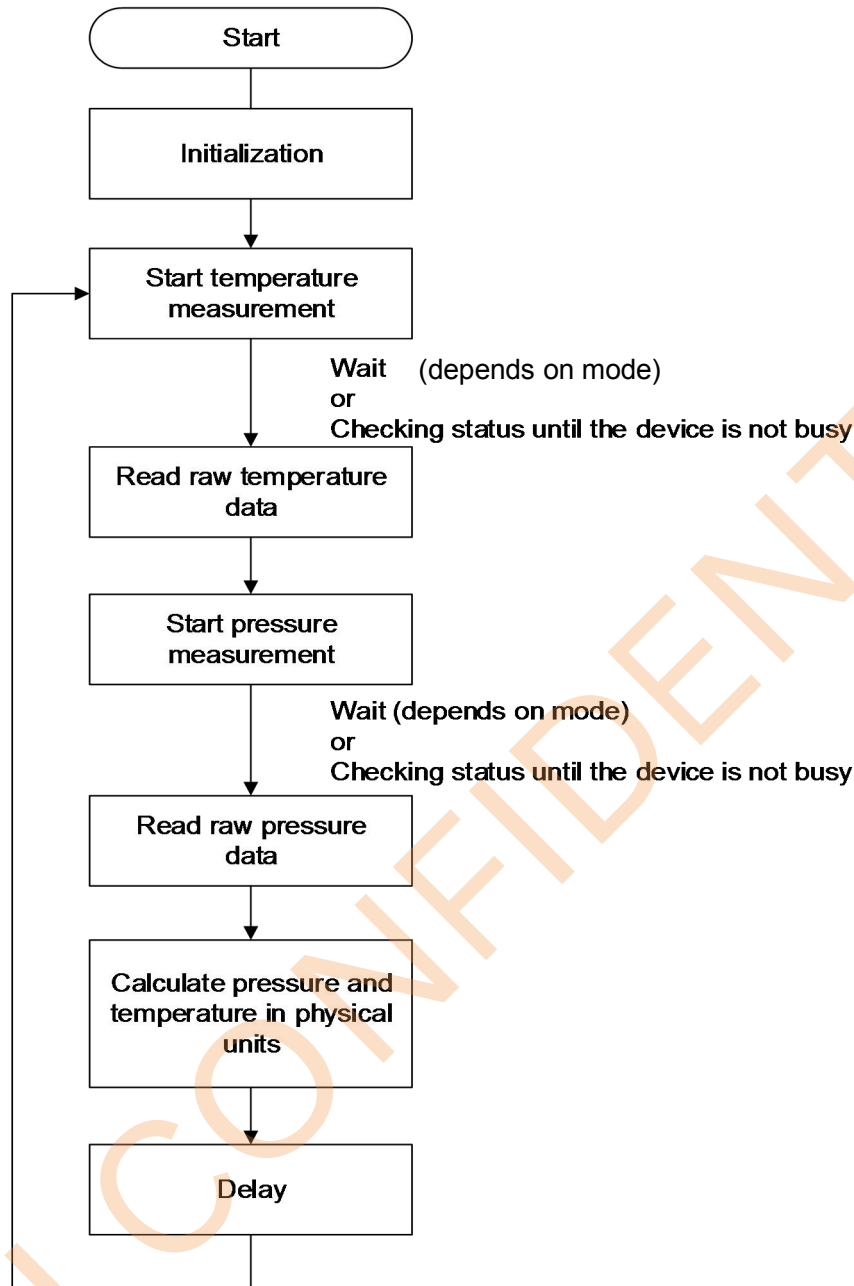
Figure 2 Measurement flow of WF5837F
