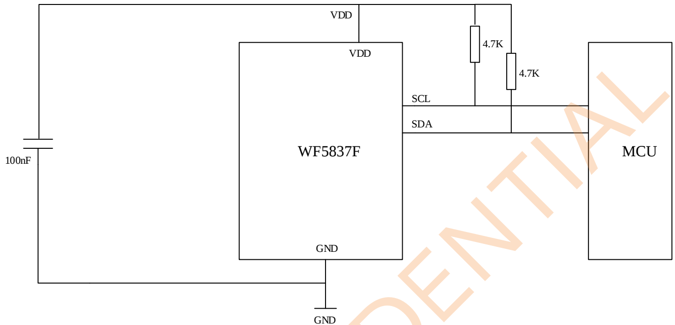
Figure 6 Typical Application (I2C Mode)
