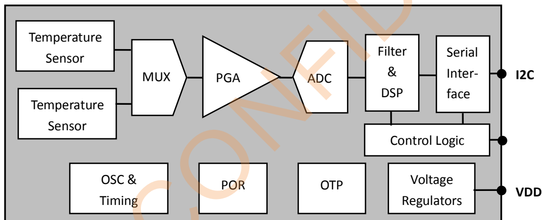
Figure 1 Block diagram of WF1214M
